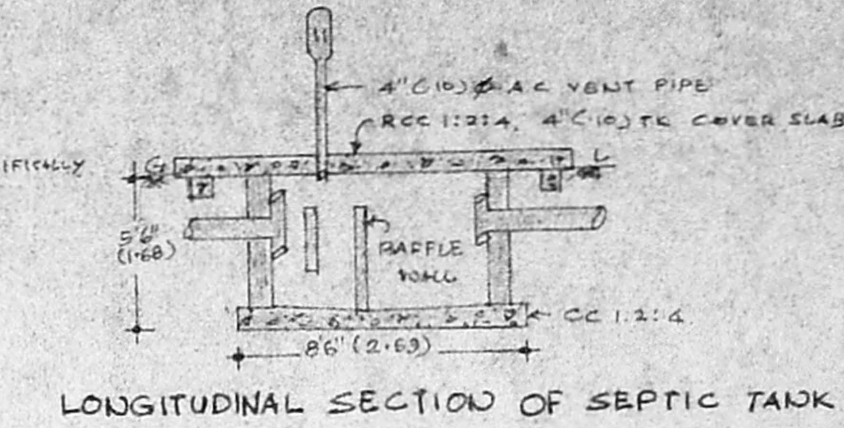
LONGITUDINAL SECTION OF SEPTIC TANK.
