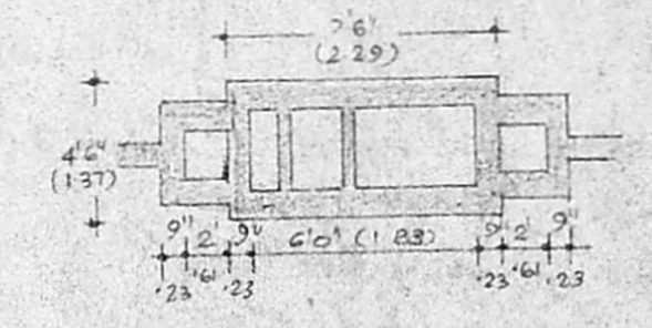
PLAN OF SEPTIC TANK. SCALE: 1:300
